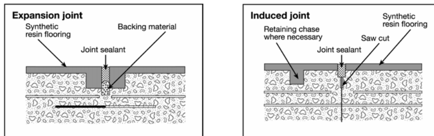
Figure 1: Movement joints
