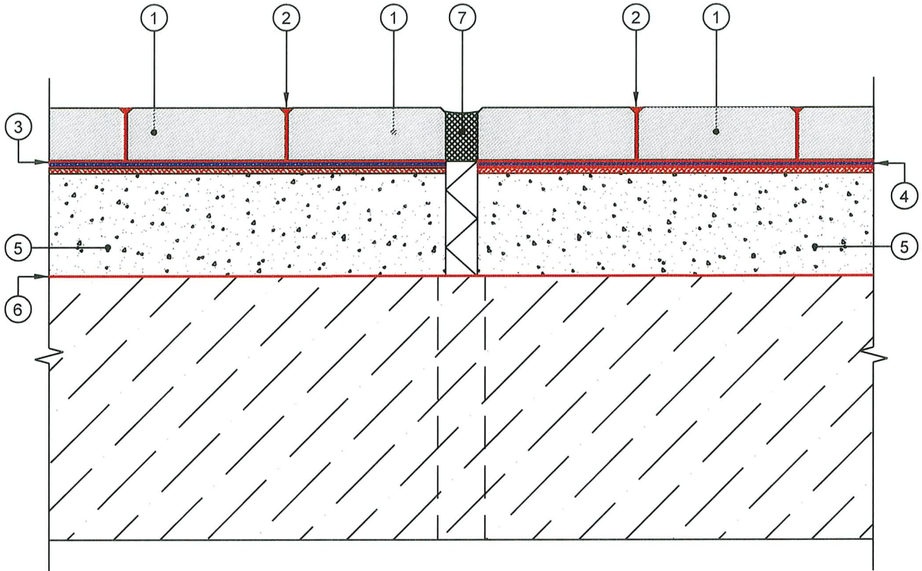
CROSS SECTION
