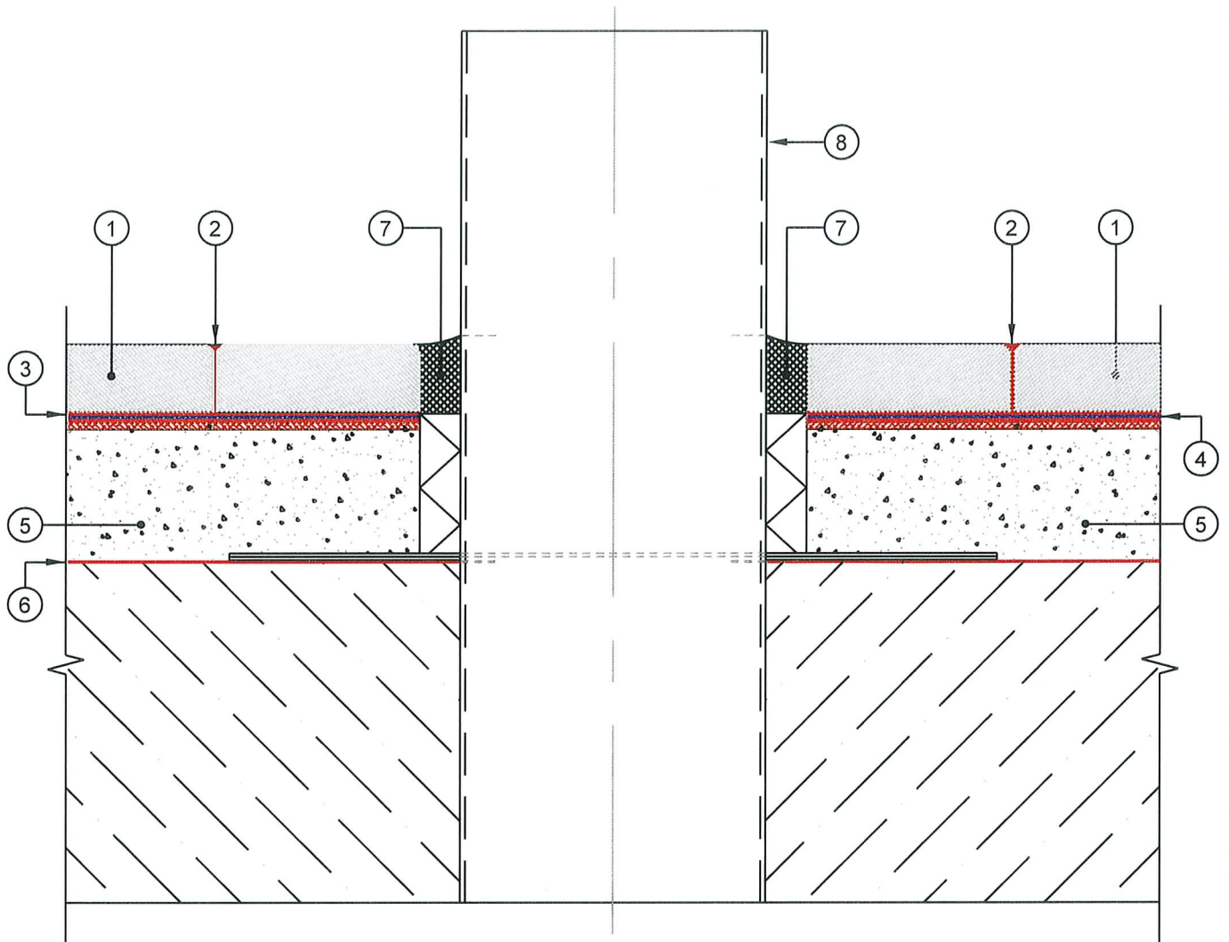
CROSS SECTION
