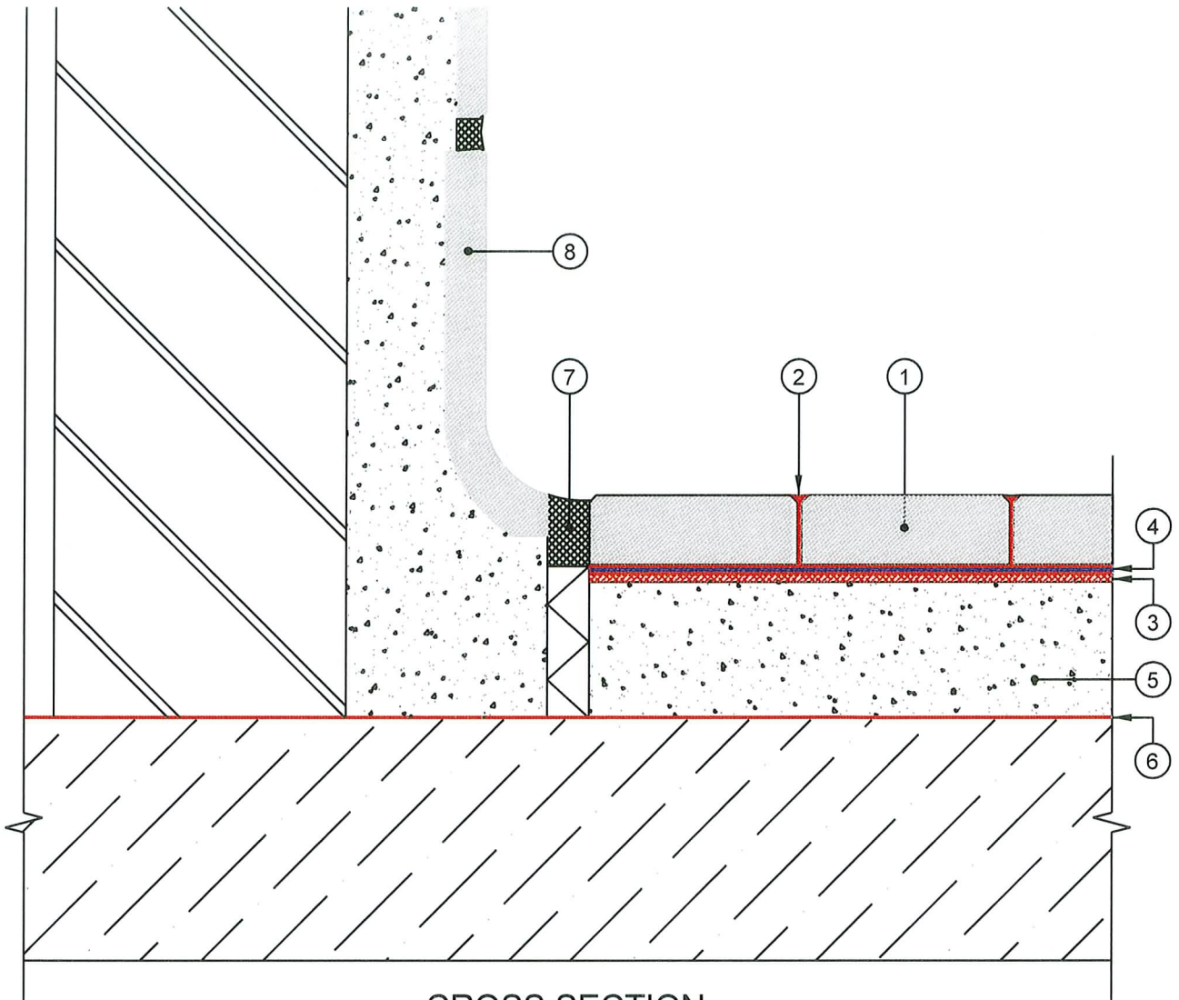
CROSS SECTION
